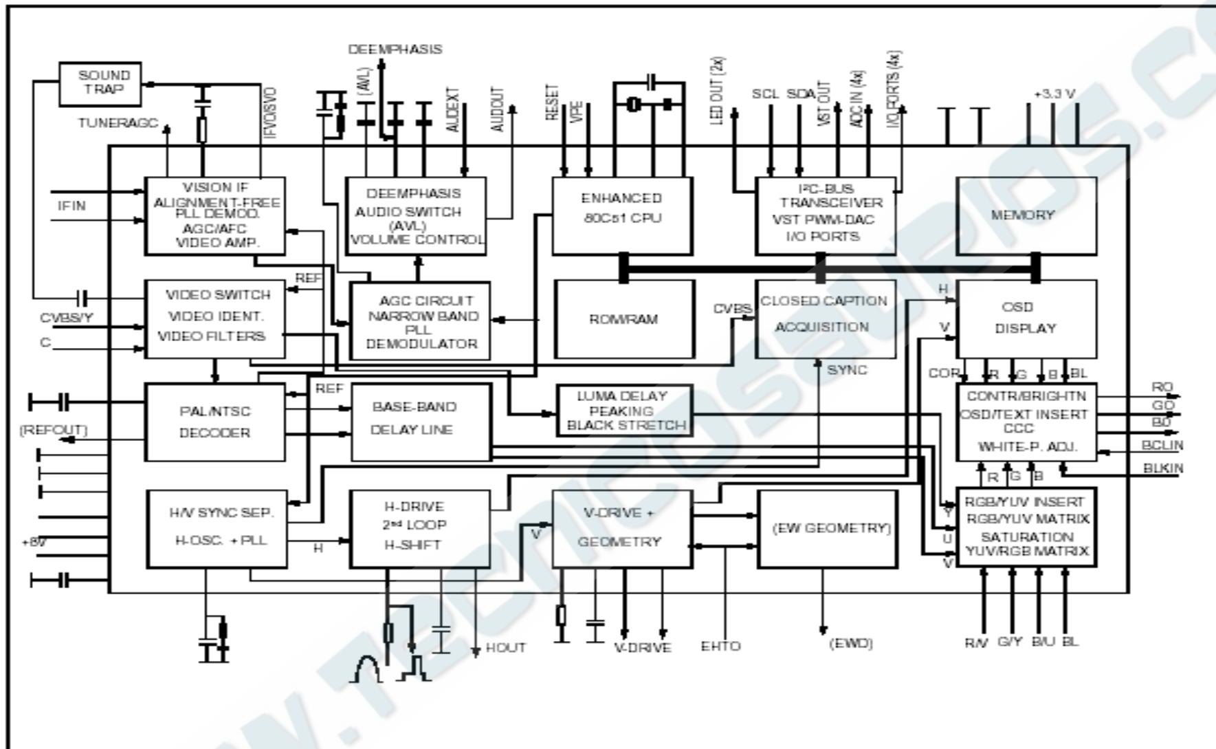
BLOCK DIAGRAM
